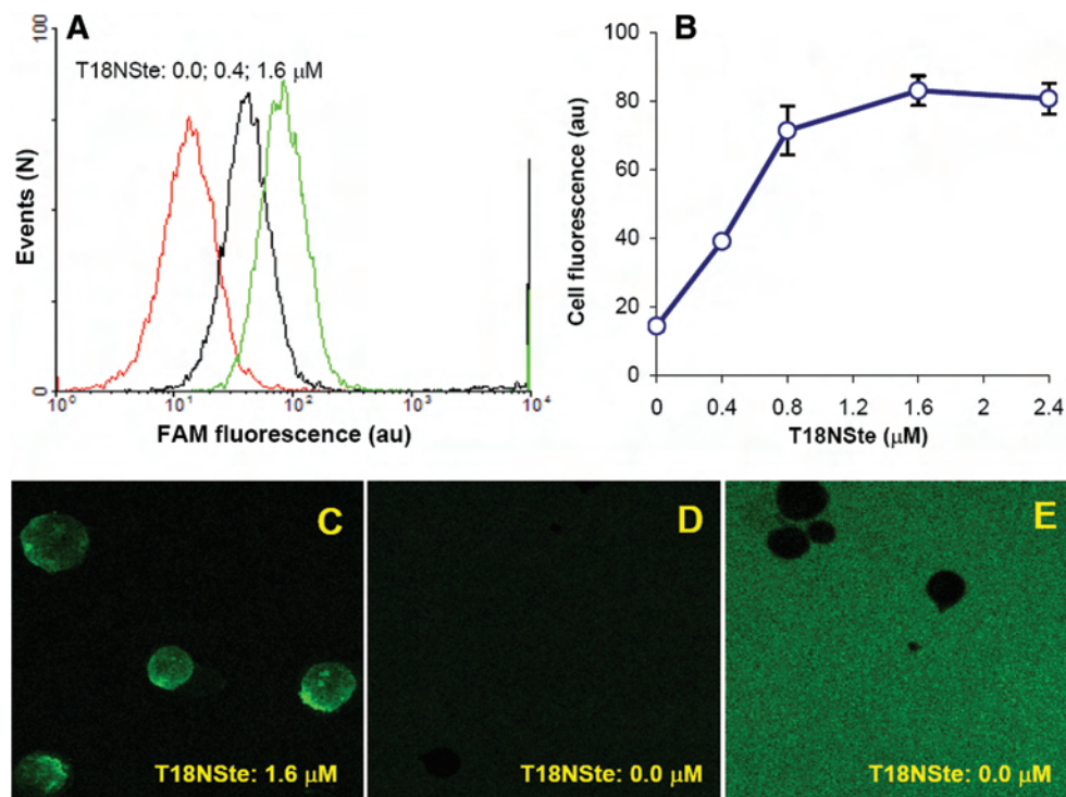
Figure 7. Hybridization of T18NSte integrated into PM with complementary A25F at the cell surface. Jurkat cells were labeled with T18NSte (0.4–2.4 \mu\text{M} ) at 37°C for 5 min, washed and incubated with complementary A25F (0.4 \mu\text{M} ) at 37°C for 5 min. Then cells were placed in water bath to cool down to 6°C during 20 min time period. (A) Histograms of cell distribution by A25F fluorescence pretreated with T18NSte at the concentration of 0.0, 0.4 and 1.6 \mu\text{M} (red, black and green lines, respectively). (B) Dose dependence of a mean A25F fluorescence intensity detected from cells on T18NSte concentration ( n = 3 ). (C–E) Microphotographs of A25F fluorescence in Jurkat cells pre-incubated with 1.6 \mu\text{M} T18NSte (C) and without T18NSte (D, E). (C, D) Instrumental conditions are similar; (E)—same as (D), but PMT gain is enhanced to demonstrate the presence of unstained cells (dark spots) on the fluorescent background of A25F.
