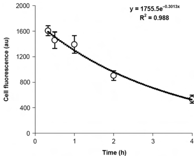
Figure 6. Time course of fluorescence quenching of FT18NSte in Jurkat cells. Cells were labeled with 0.2 \mu\text{M} FT18NSte for 10 min at 37°C in serum-free RPMI, washed and cultured in complete RPMI medium. Fluorescence was evaluated by flow cytometry.
